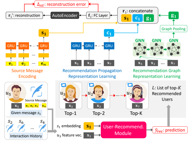
Figure 1: The overview of the proposed RecMR framework.
